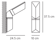
Teseo parete FLUO 1x11W (G 23) – TC-S
