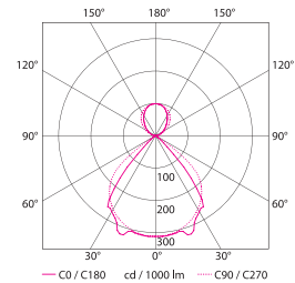
d-RABBIT 1xT16 54W
