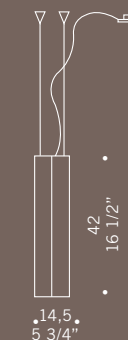
CARRÈ S1GD 1x70W E27 alogeno chiara clear halogen 1x26W E27 fluorescente fluorescent cavo elettrico 200 cm cables length 200 cm
