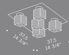
OTTO X OTTO P5 5x40W G9 alogeno bispino halogen bi-pin
