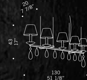
ELORO S5L SHADE 5x40W E14 sferetta chiara little sphere
