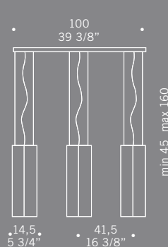
CARRÈ S3PL 3x70W E27 alogena chiara clear halogen 3x26W E27 fluorescente fluorescent
