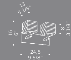
OTTO X OTTO A2 2x60W G9 alogeno bispino halogen bi-pin
