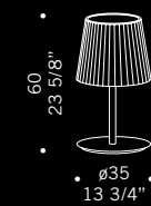
LUMÈ T1 1x60W E27 Globolux chiara clear Globolux 1x70W E27 alogeno chiara clear halogen
