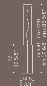
CARRÈ S1P 1x70W E27 alogeno chiara clear halogen 1x26W E27 fluorescente fluorescent
