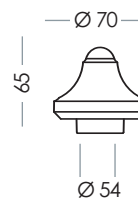
Terminale in plastica per palo Ø 60x3 Plastic pole top end finial Ø 60x3
