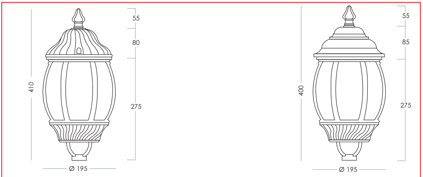
ART. 5091I-A-I Rame grezzo - Raw copper
