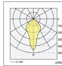
n° 86 FILIPA G HIT-T 70W con reflector S2 / with S2 reflector \eta=54.200\%
