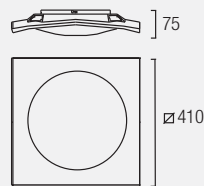
15-2391-21-E9 R7s L=118 Max. 200W HALOGEN OSRAM included
