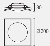
15-2390-21-E9 R7s L=78 Max. 150W HALOGEN OSRAM included
