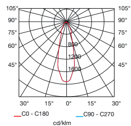
Par-30 75W
