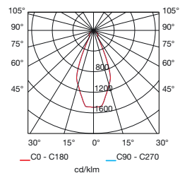
GU-10 50W
