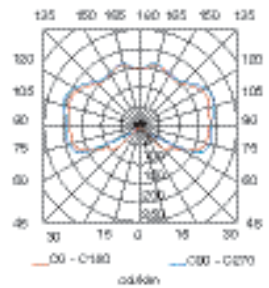
E-27 100W
