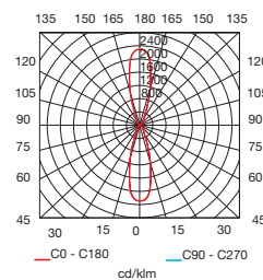
GU-10 50W
