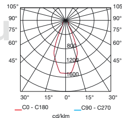
GU-10 50W
