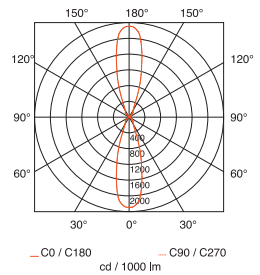
GU-10 50W
