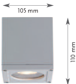
Ceiling Bracket (fix)
